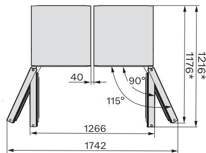
KS4383ED N, KS4383DD N, FNS4382E N, FNS4382D N, Nordic, installation sketch, Side-by-Side
